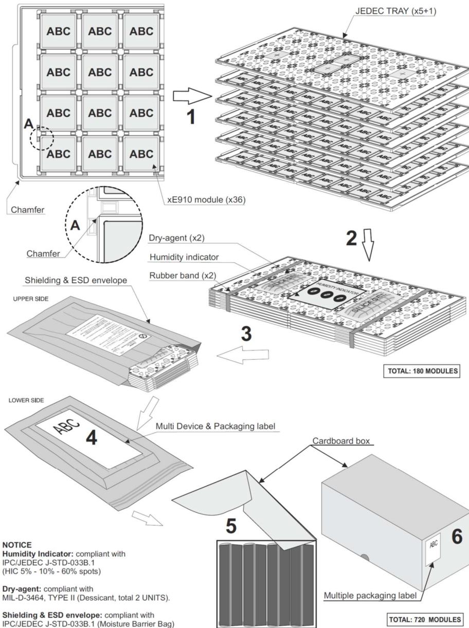
Figure 38: Packing
