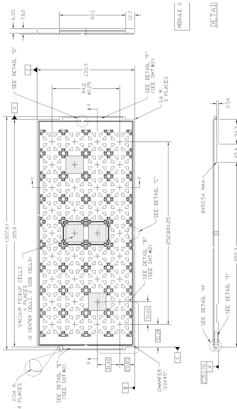
Figure 39: Tray Drawing
