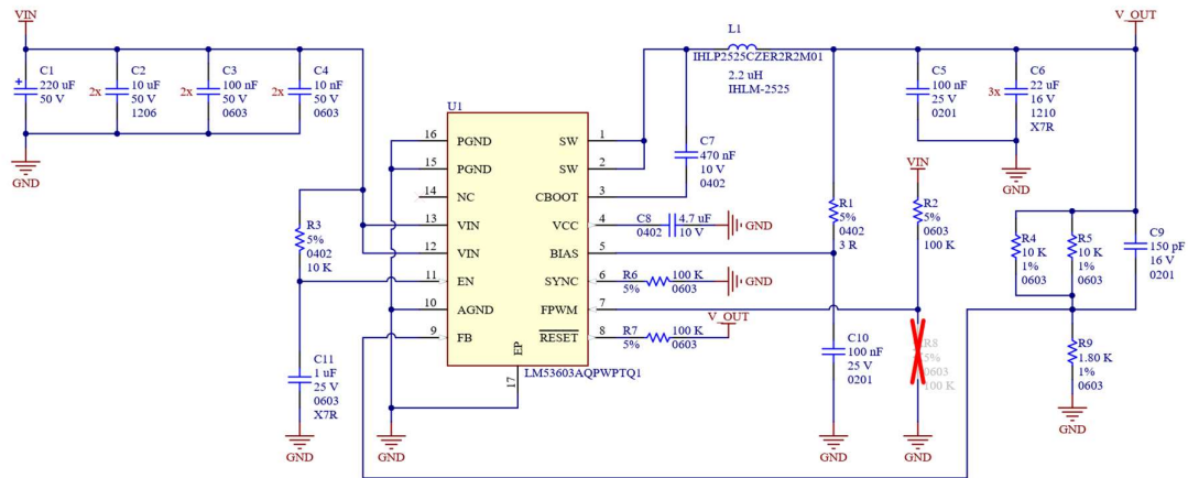
Figure 15: Example of Switching Regulator with 12V Input
