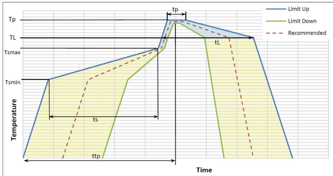
Figure 36: Solder Reflow Profile
