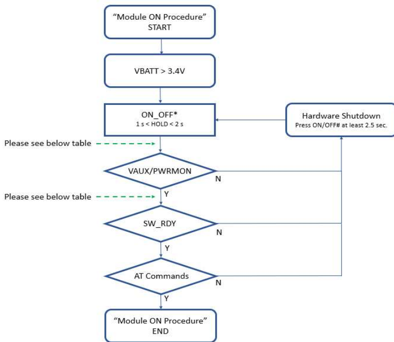
Figure 6: Turn-on Procedure
