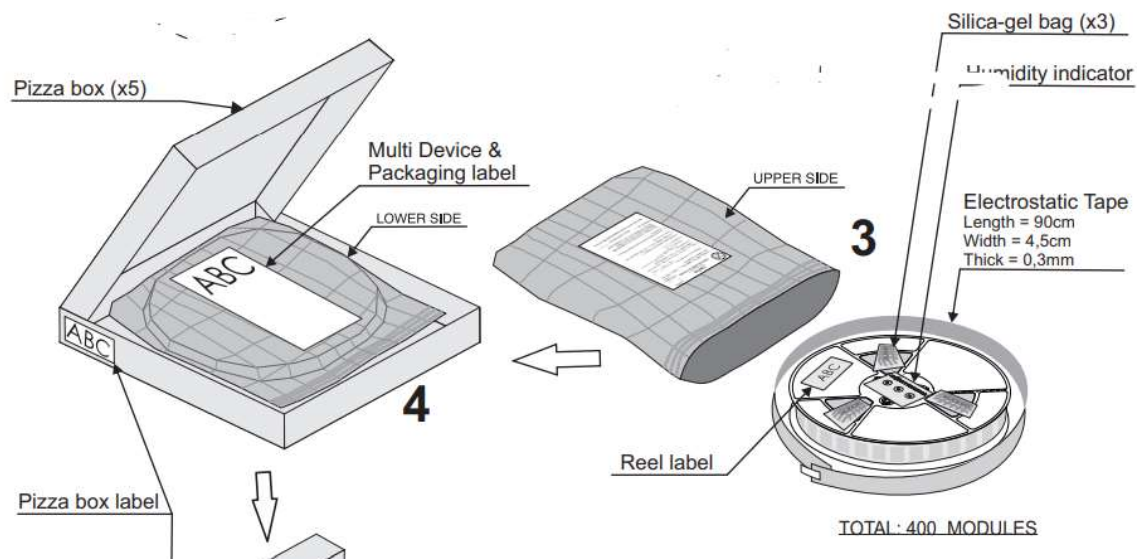
Figure 50: LE910Cx-WWX(D) Reel Box Detail
