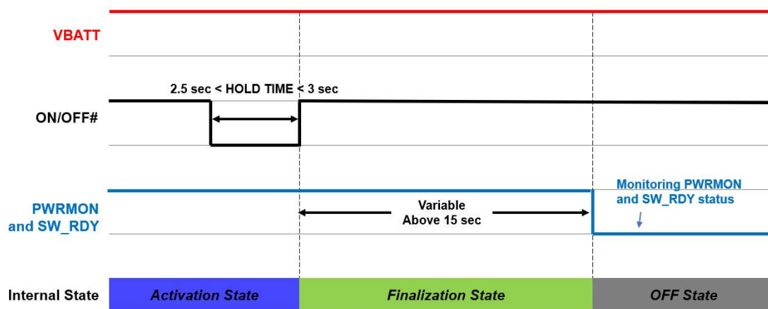
Figure 9: Hardware Shutdown
