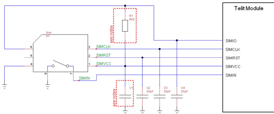
Figure 37: SIM Schematics
