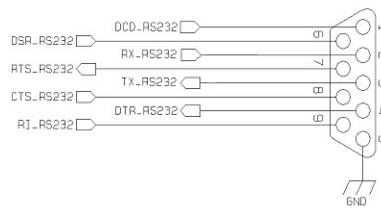
Figure 17: RS232 Serial Port Lines Connection Layout
