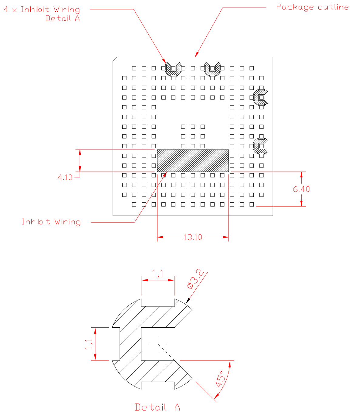
Figure 32:: Inhibit Wiring Area
