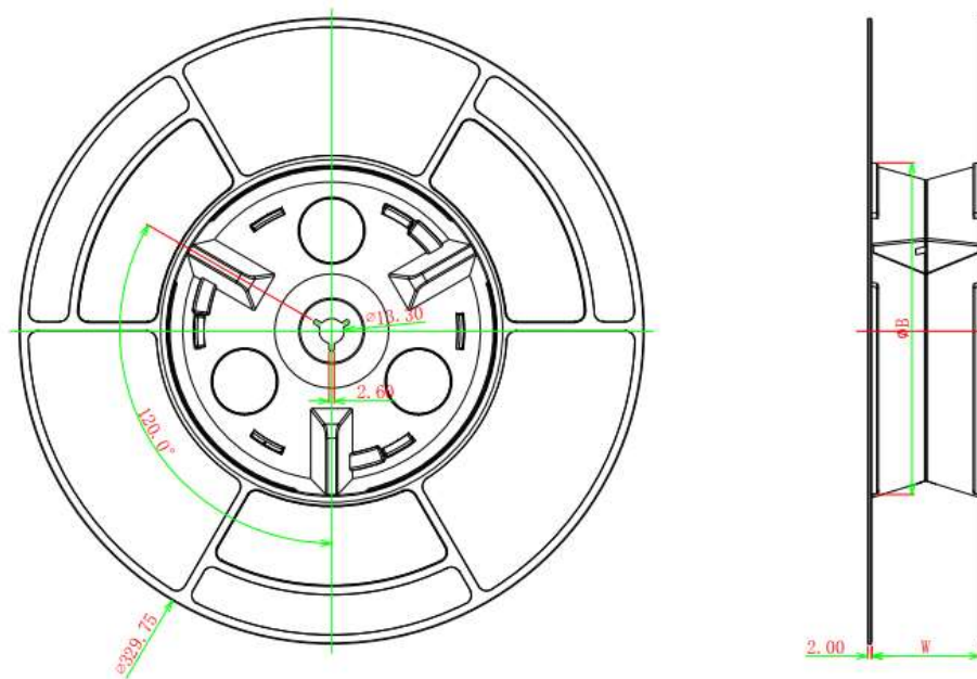
Figure 49: LE910Cx-WWX(D) Carrier Tape Detail
