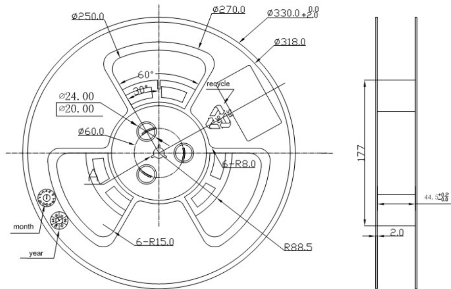
Figure 44: Reel Detail
