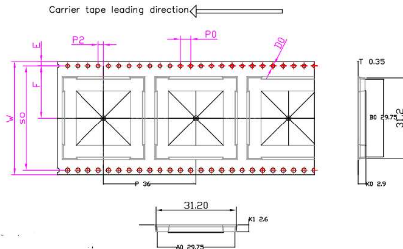
Figure 48: WWX Carrier Tape Detail
