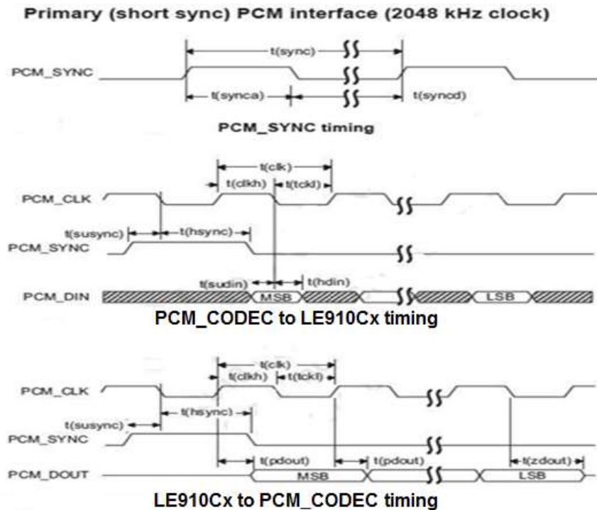
Figure 20: Primary PCM Timing
