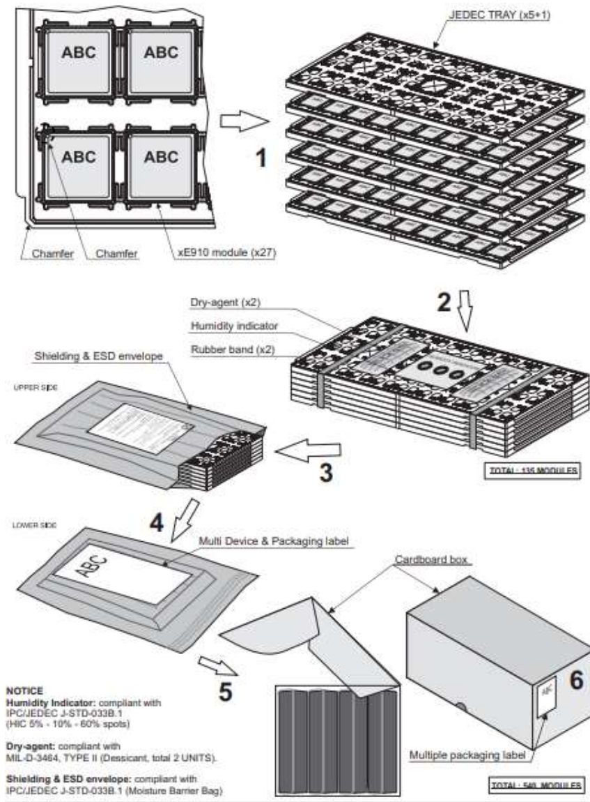
Figure 40: Packing
