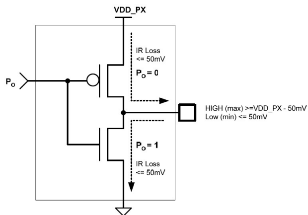
Figure 23: GPIO Output Pad Equivalent Circuit
