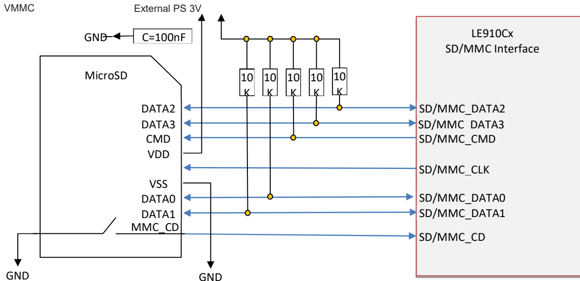
Figure 19: SD/MMC Interface Connectivity
