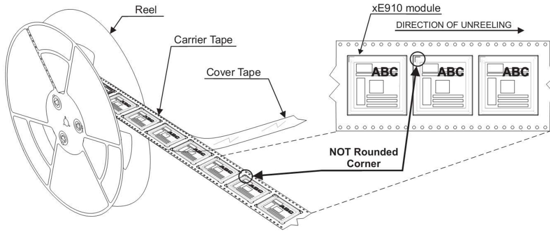
Figure 42: Module Positioning into the Carrier
