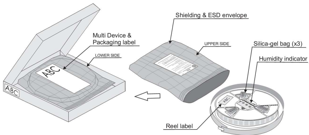
Figure 46: Reel Box Detail
